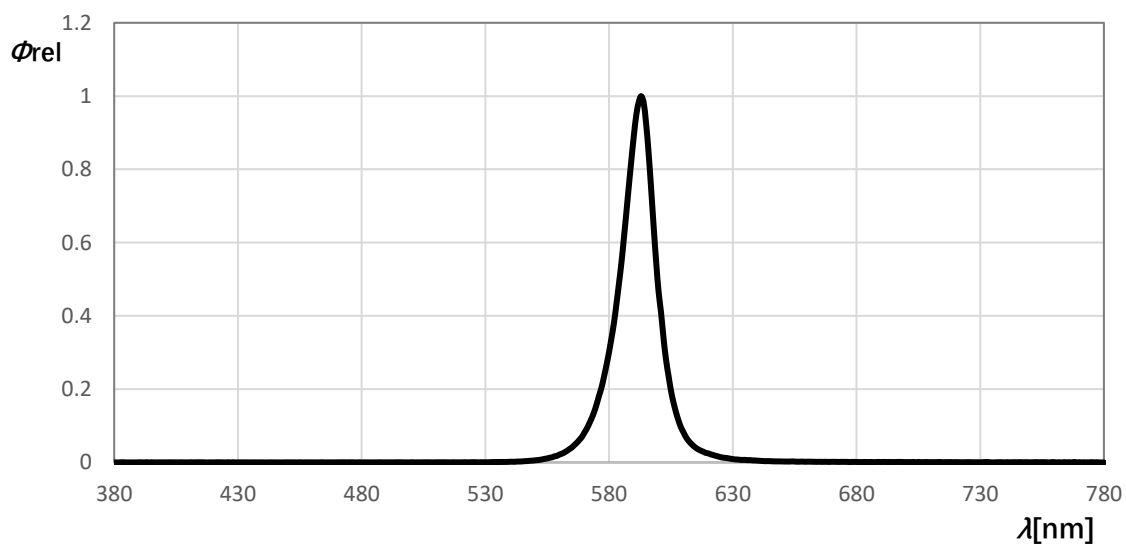
Fig 2. 相对发光光谱 Relative Spectral Distribution vs. Wavelength
