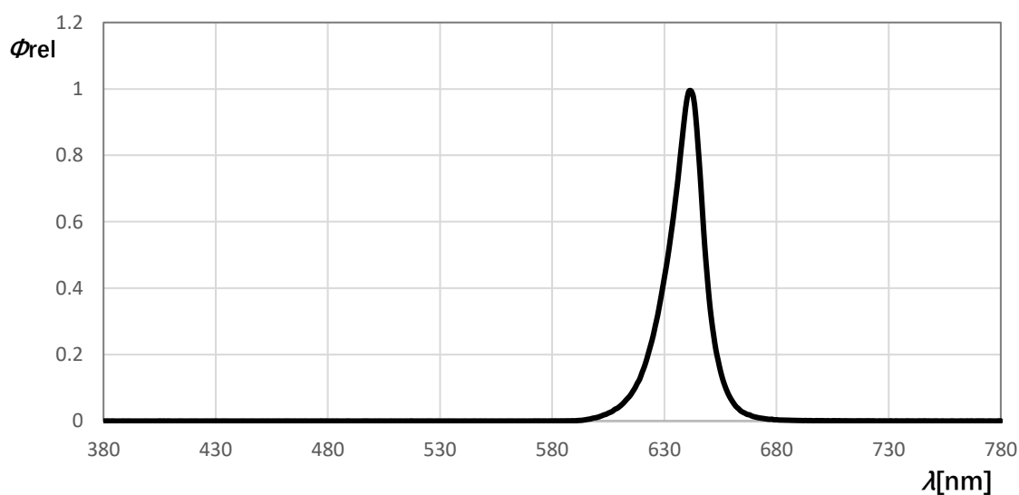
Fig 2. 相对发光光谱 Relative Spectral Distribution vs. Wavelength
