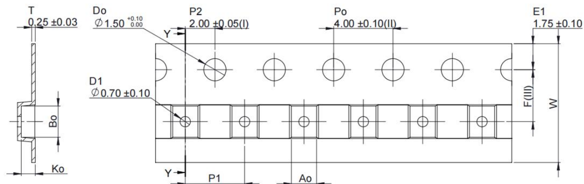
SECTION Y-Y
