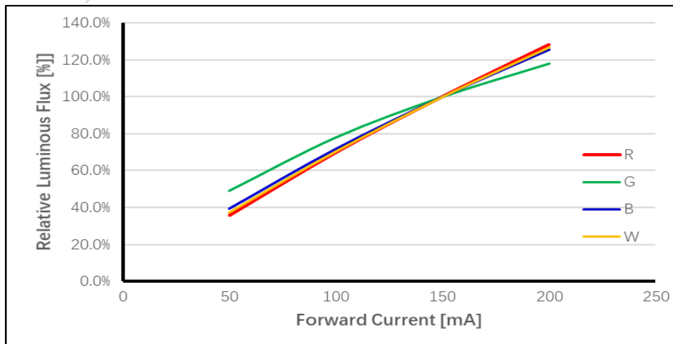
c)、Forward Current vs. Relative Luminous Flux, T_a=25^\circ\text{C}
